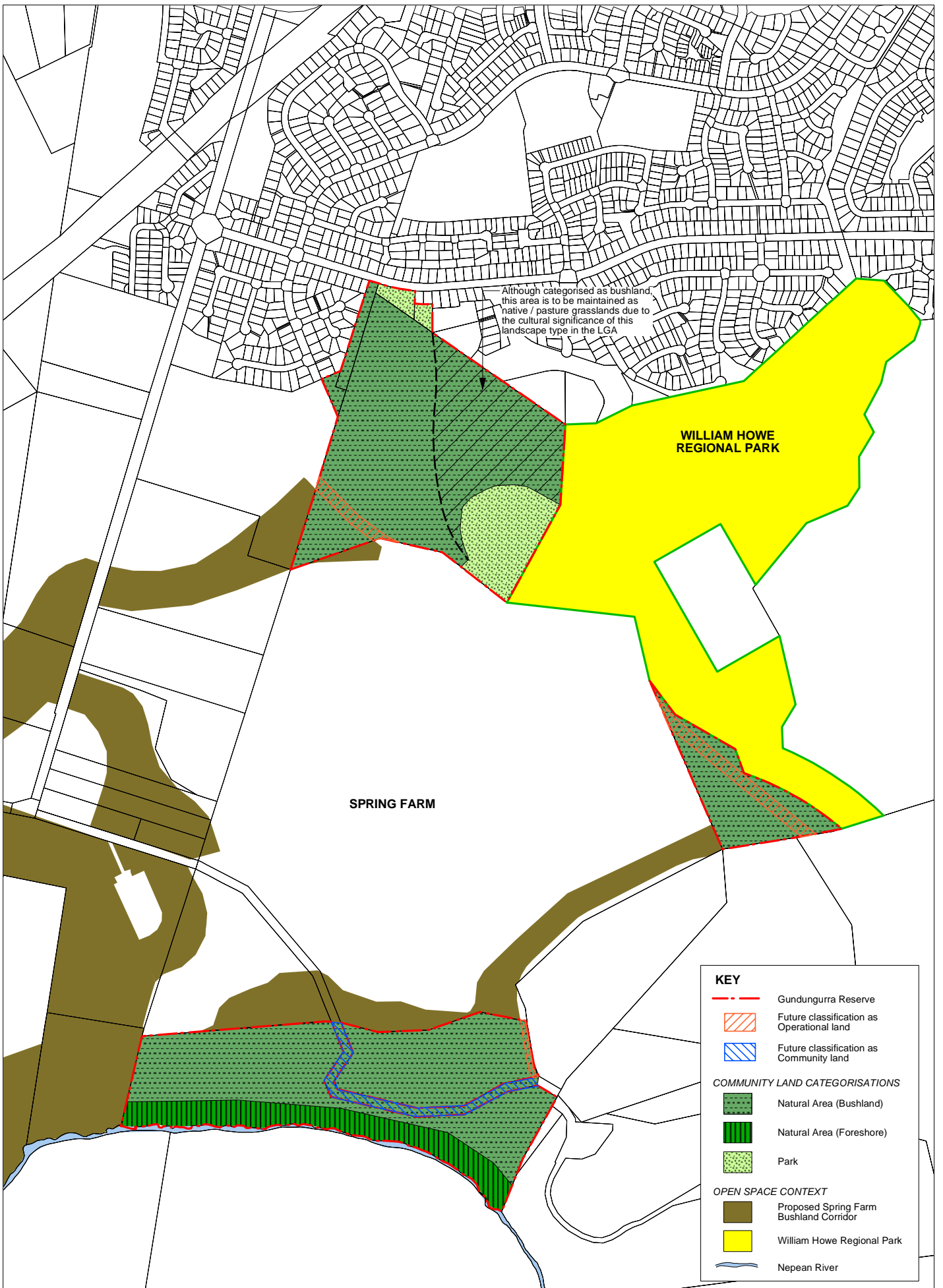
Figure 5.1 Land Categorisation
